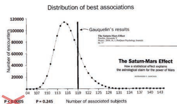
Figure 1—Distribution of best associations. In one million iterations the exact number of subjects in the group that had the strongest association with a planet in two sectors was calculated. Gauquelin's results fall just slightly to the right of the peak of the distribution.
